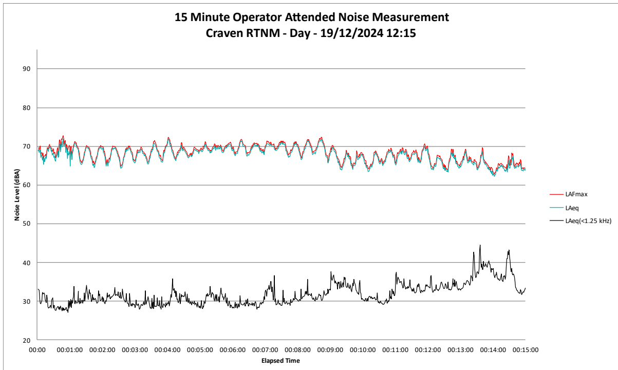
Figure B26 – Day Period – ‘Craven RTNM’ Operator Attended Noise Survey Results
