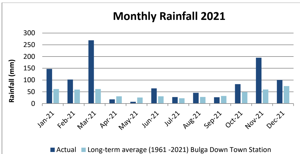
FIGURE 5 MONTHLY RAINFALL – SOUTHERN BA
