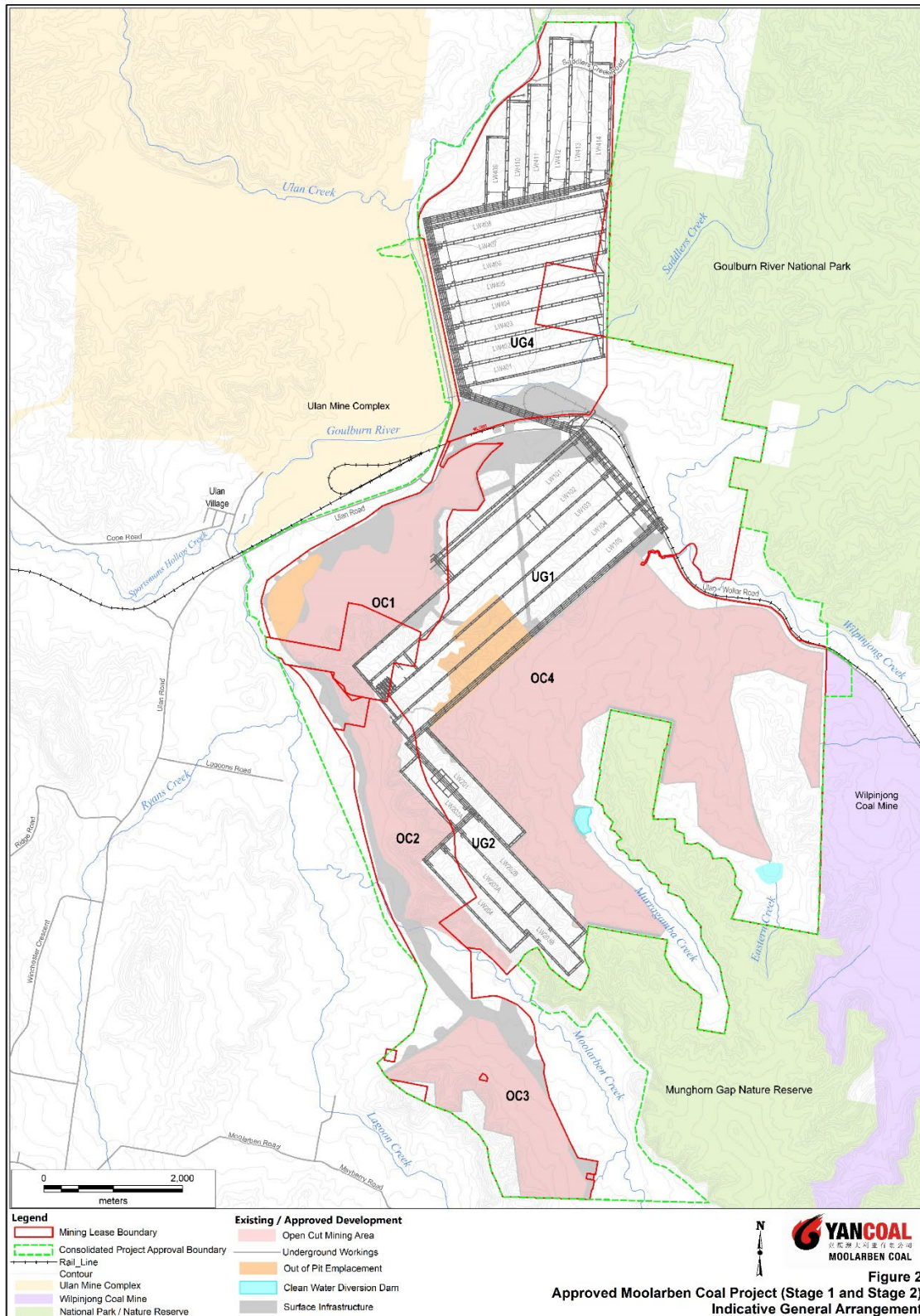
Figure 2: General Arrangement
