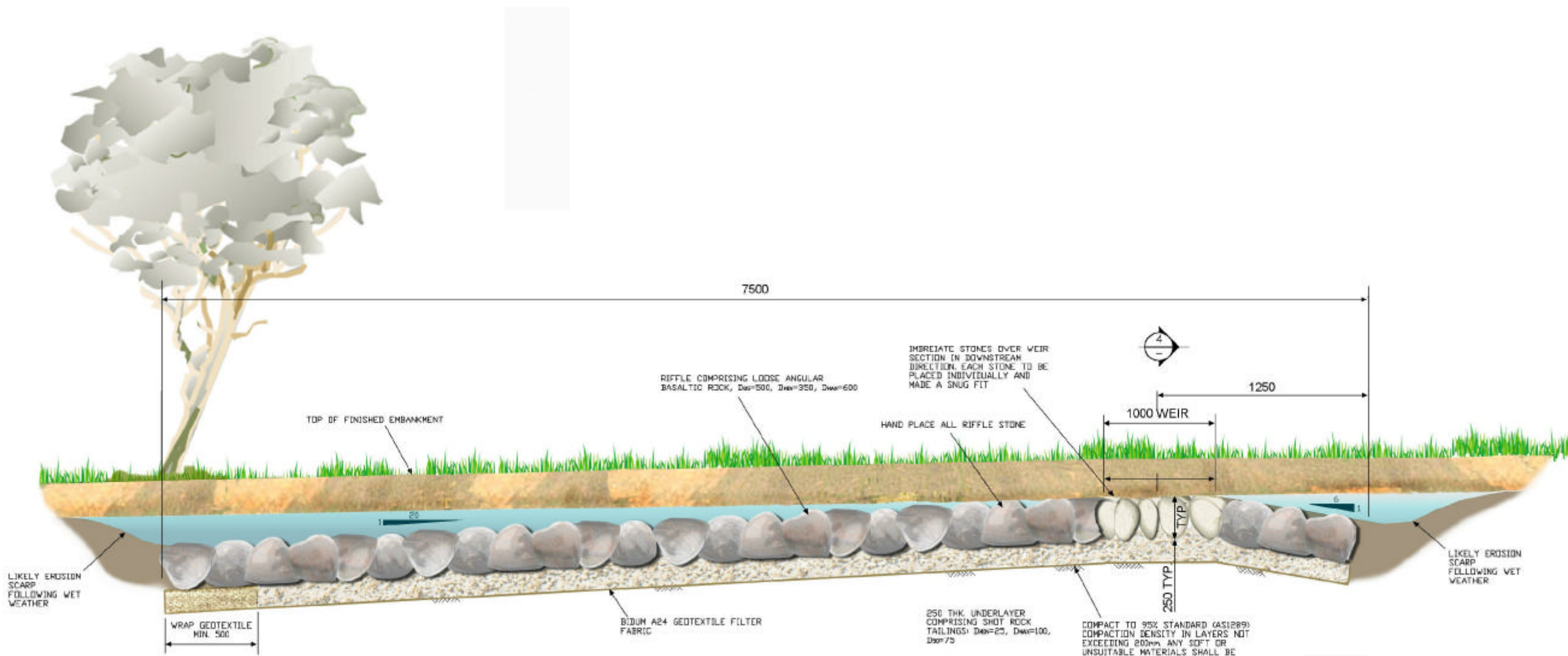
TYPICAL RIFFLE SECTION N.T.S.
