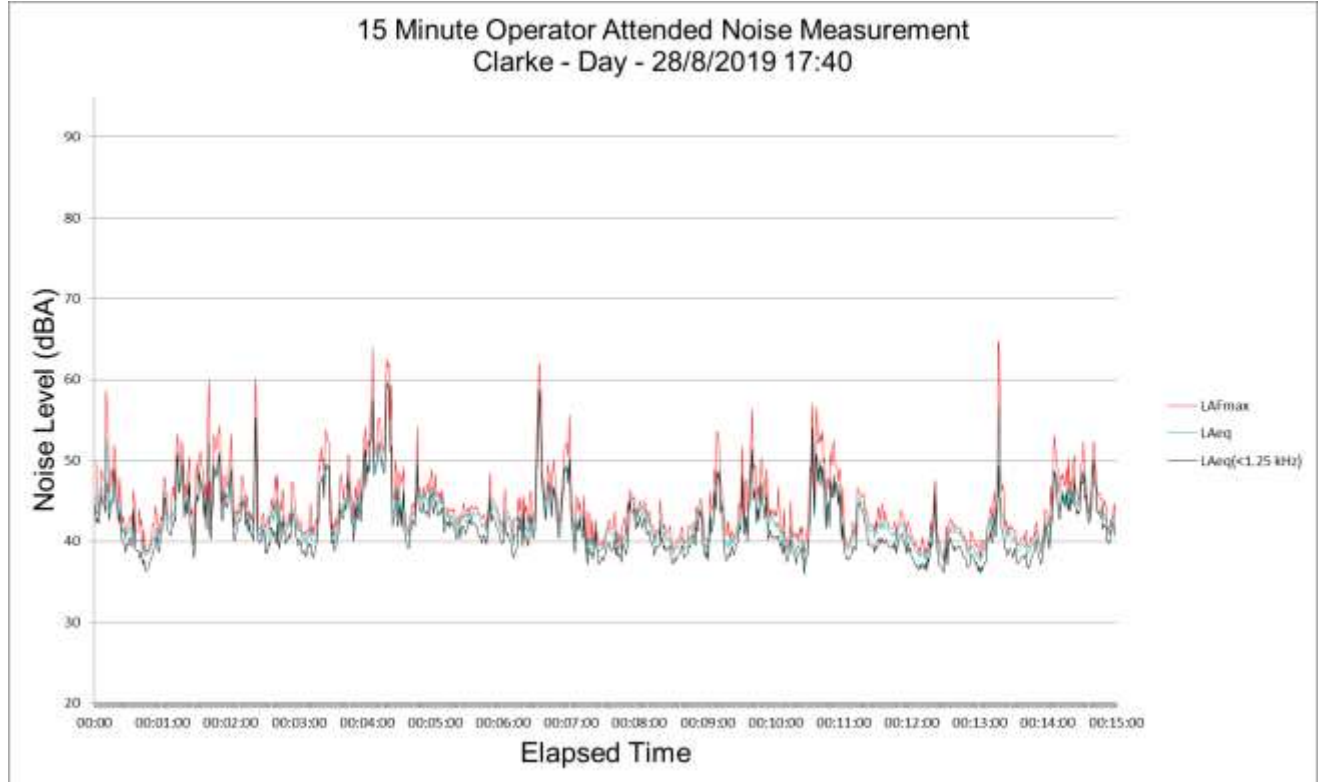
Figure B4 – Day Period – ‘Clarke’ Operator Attended Noise Survey Results
