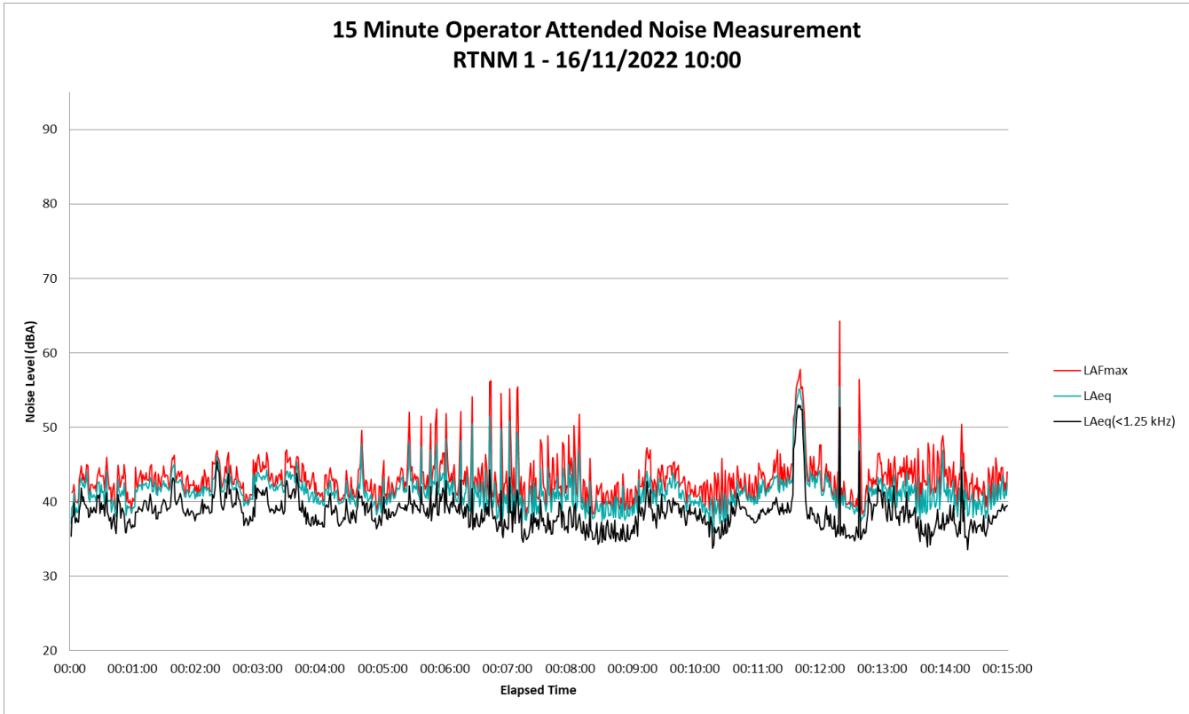
Figure B26 – RTNM1 – Noise Level Trend – Q4 2022 RTNM 15 Minute Noise Measurement
