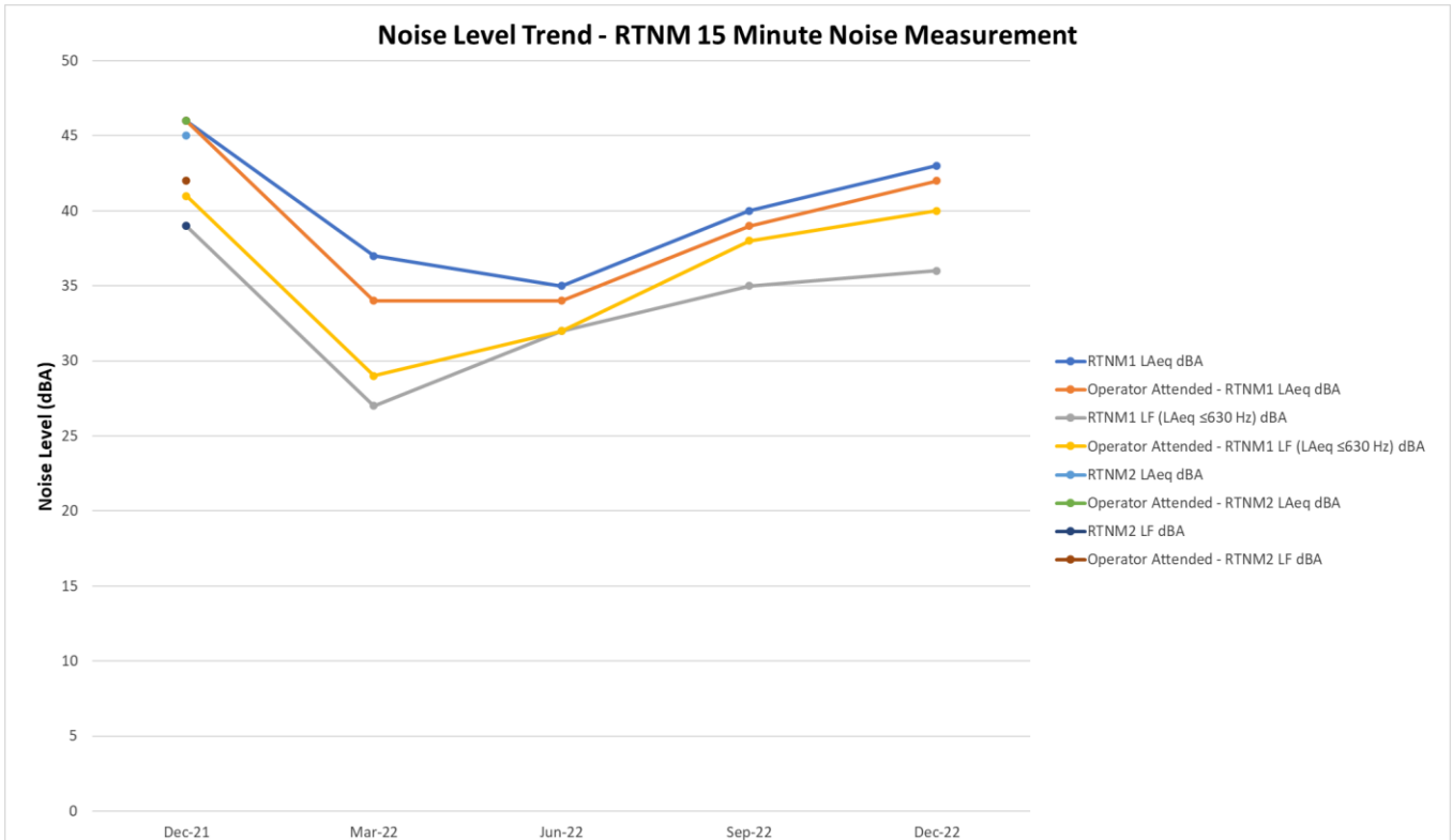
Figure B26 – RTNM1 – Noise Level Trend – Q4 2022 RTNM 15 Minute Noise Measurement
