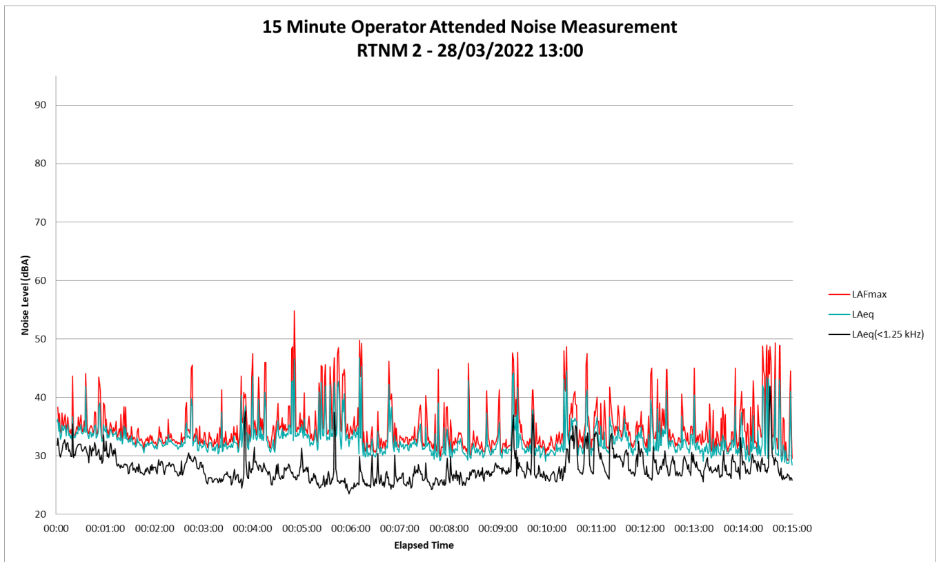
Figure B25 – RTNM2 Operator Attended Noise Survey Results
