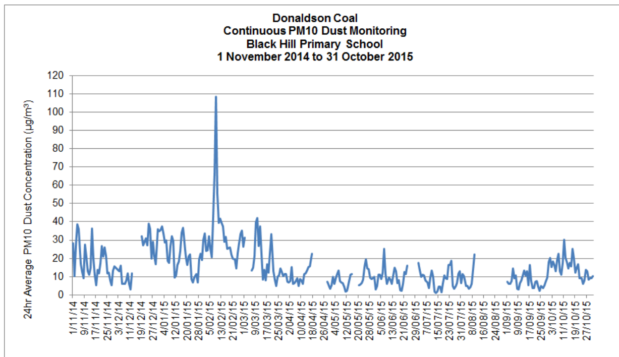
Figure 2: Results of DustTrak Continuous Monitoring
