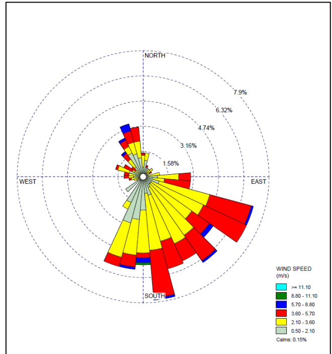
Figure 2: Charlton Ridge Wind Rose – February 2023
