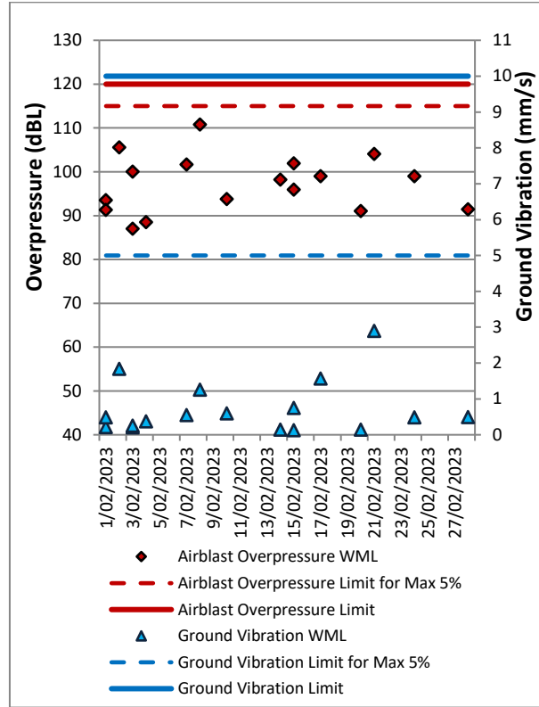
Figure 14: Warkworth Blast Monitoring Results - February 2023
