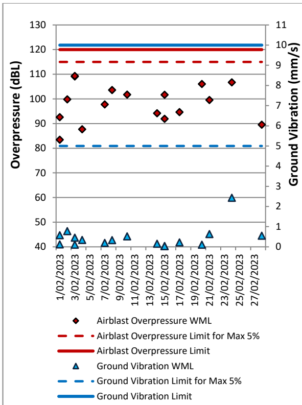
Figure 12: Wollemi Peak Road Blast Monitoring Results – February 2023
