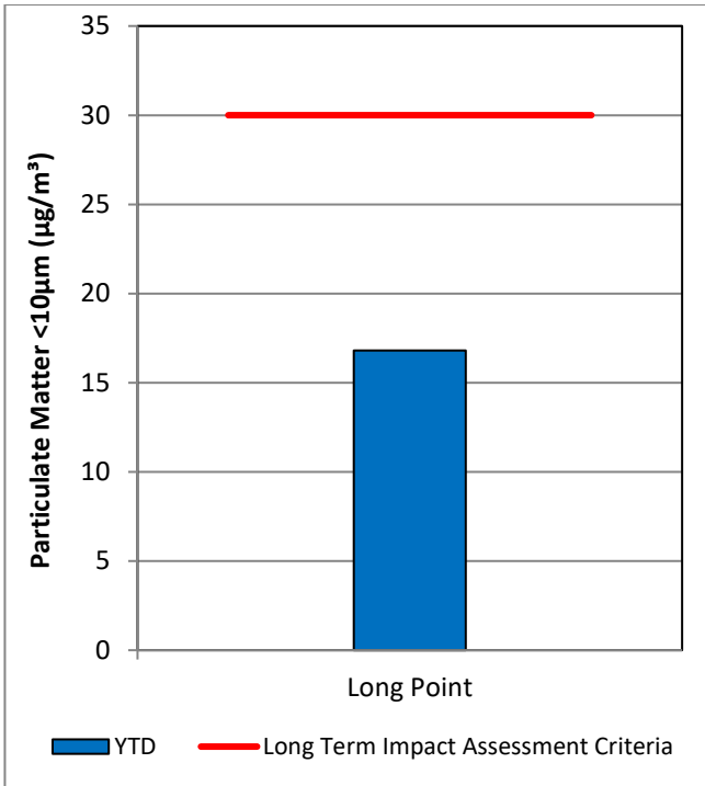
Figure 6: Annual Average PM 10 – February 2023
