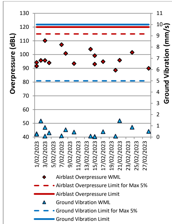
Figure 13: Wambo Road Blast Monitoring Results – February 2023
