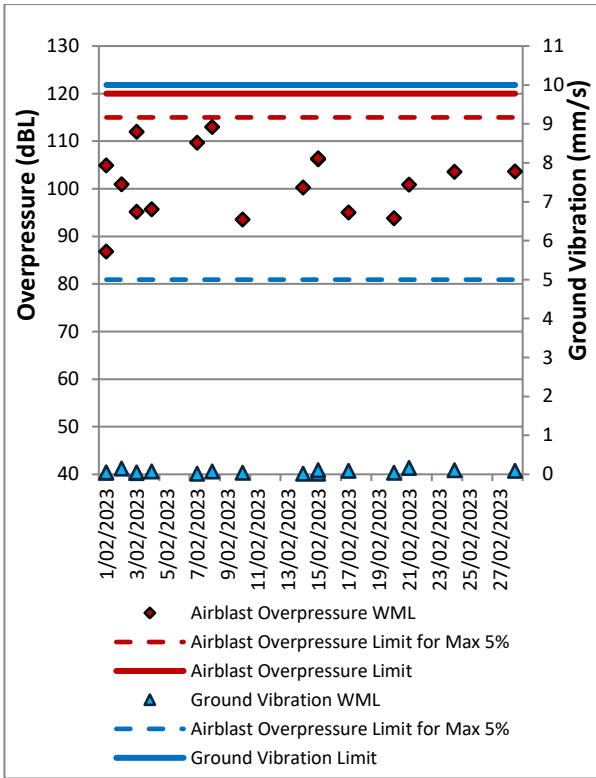
Figure 11: MTIE Blast Monitoring Results – February 2023
