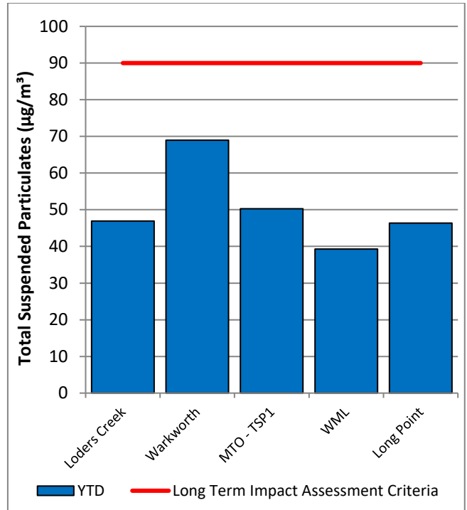
Figure 7: Annual Average Total Suspended Particulates – February 2023
