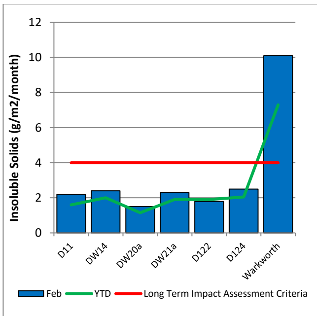
Figure 4: Depositional Dust – February 2023
