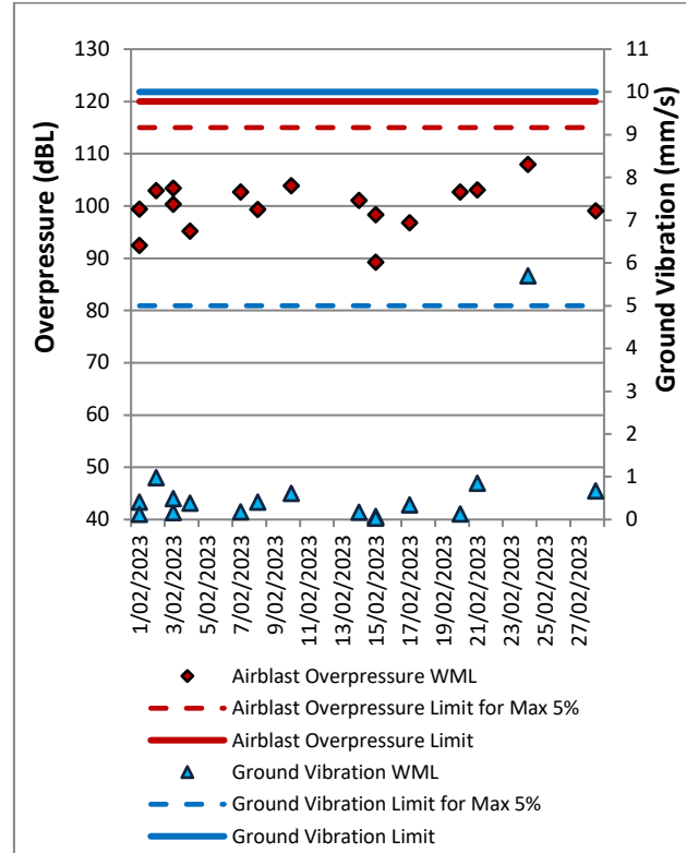
Figure 10: Bulga Village Blast Monitoring Results – February 2023
